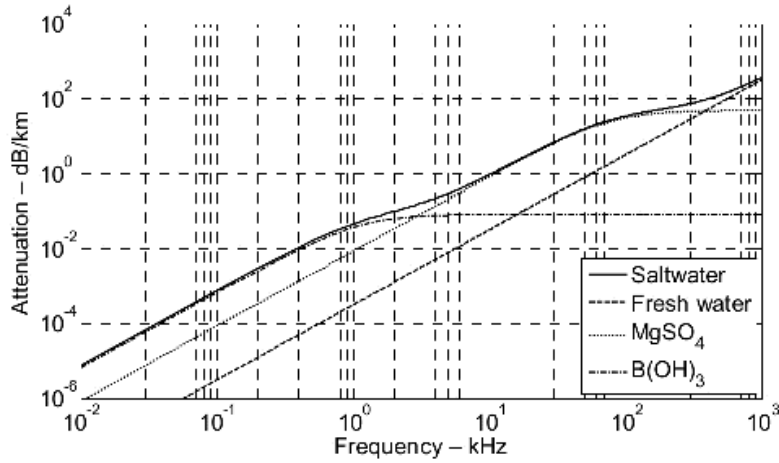
Figure 8. Acoustic absorption (dB/km) for fresh water and saltwater, plotted as a function of frequency (kHz) for water temperature of 10°C, atmospheric pressure of one atmosphere (surface), salinity of 35 pro mille, and pH value of 7.8. The various contributions to the absorption are also indicated.
