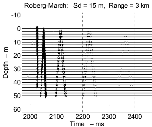
Figure 20. Time responses as function of receiver depth at a fixed horizontal distance of 3 km from a source at 15 m depth.
