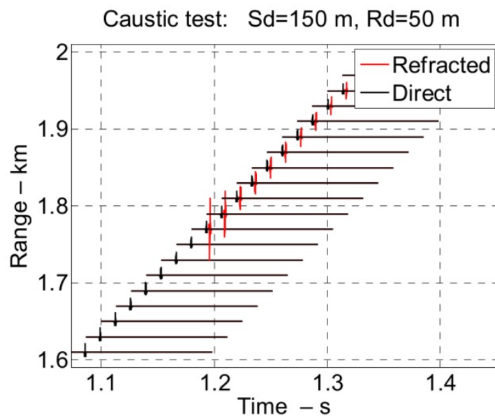
Figure 15. Time responses around the caustic at 1.76 km. The transmitted signal is a Ricker pulse with peak frequency of 200 Hz.
