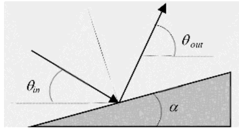
Figure 2. A ray with horizontal angle \theta_{in} strikes a plane with inclination \alpha , the reflected ray is changed to \theta_{out} .
