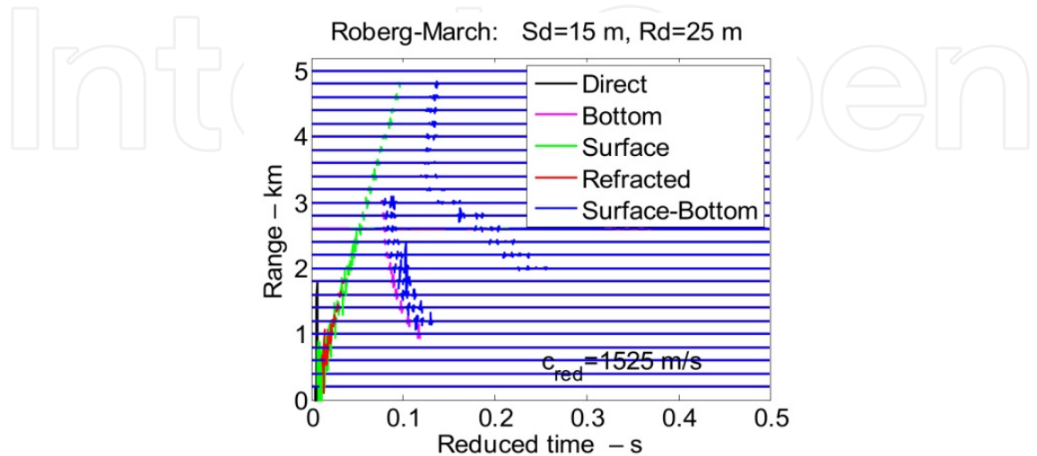
Figure 19. Time responses as function of range for receivers at depths of 25 m with a source at 15 m.
