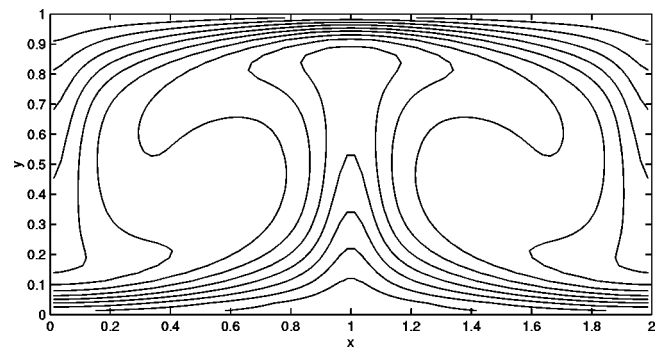
FIG. 7. Temperature contours at Ra=50000.
