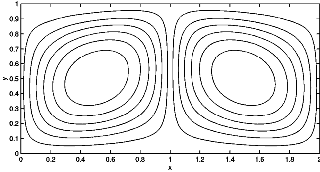
FIG. 8. Stream function contours at Ra=50\,000 .
