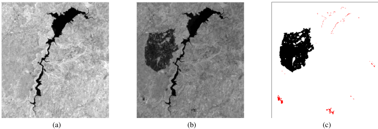
Fig. 6. Dataset C: images of Lake Omodeo and surrounding area (Italy) acquired by the Operational Land Imager sensor of the Landsat 8 satellite: (a) channel 5 of the image acquired in July 2013; (b) channel 5 of the image acquired in August 2013; (c) change reference map indicating the burned area extension (black) and other minor changes related to clouds and water (red).
