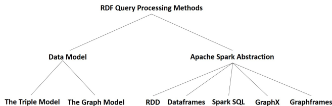
Fig. 1. A taxonomy presenting the dimensions for organizing RDF query processing methods.
