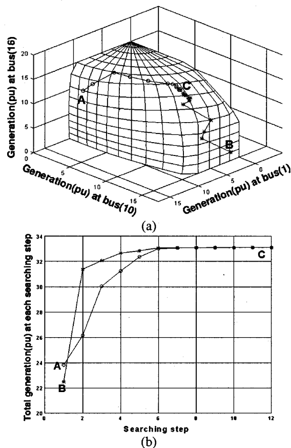
Fig. 2. Searching the K_{PG} for the maximum generation capability: (a) On the surface, and (b) at each step.
