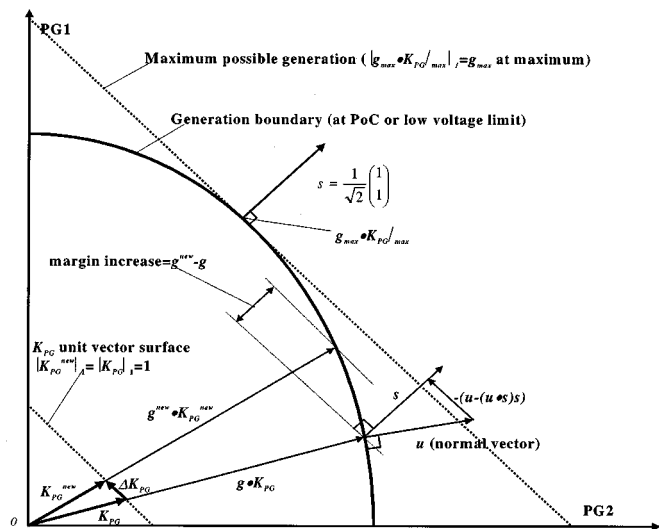
Fig. 1. The search algorithm.
