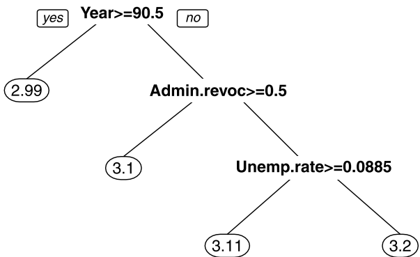
Fig. 10 Estimated RE-EM tree for the logged fatality rate in the traffic data
