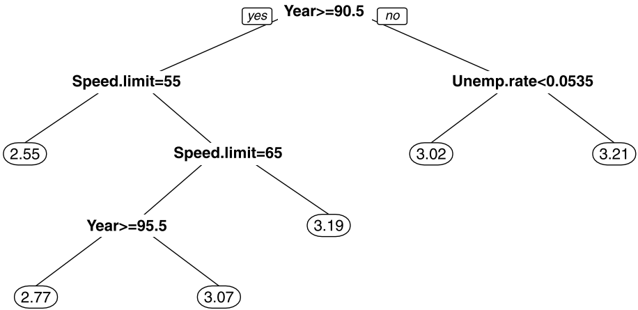
Fig. 9 Estimated tree without random effects for the logged fatality rate in the traffic data
