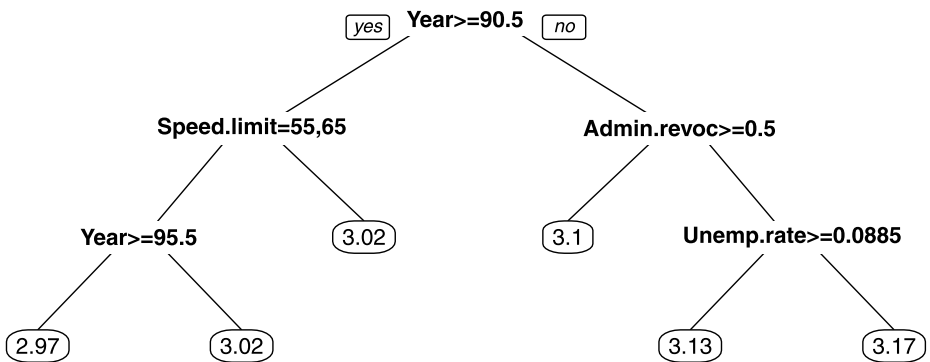
Fig. 11 Estimated RE-EM tree with autocorrelation for the logged fatality rate in the traffic data
