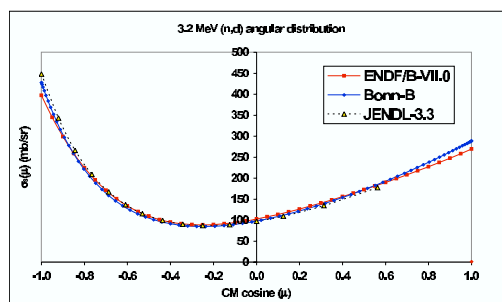
Fig. 7. As in figure 5 for 3.2 MeV neutrons.
