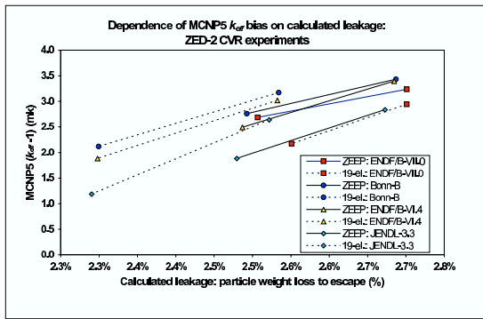
Fig. 8. MCNP5 ZED-2 CVR k_{\text{eff}} bias results for selected CVR experiments: dependence on calculated neutron leakage.
