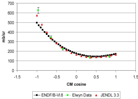
Fig. 2. As in figure 1 for 1.0 MeV neutrons. Data from Elwyn et al. [2].
