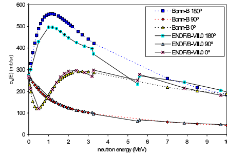
Fig. 4. Differential cross section (mb/sr) for scattering of neutrons from deuterium, at 0°, 90° and 180°. AGS calculations with the Bonn-B NN interaction, compared to the ENDF/B-VII.0 library.
