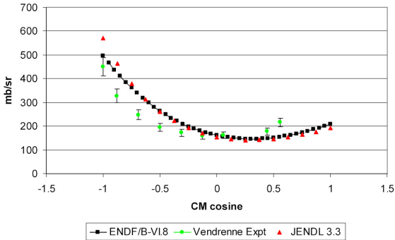
Fig. 3. As in figure 1 for 1.2 MeV neutrons. Data from Vendrenne [3].
