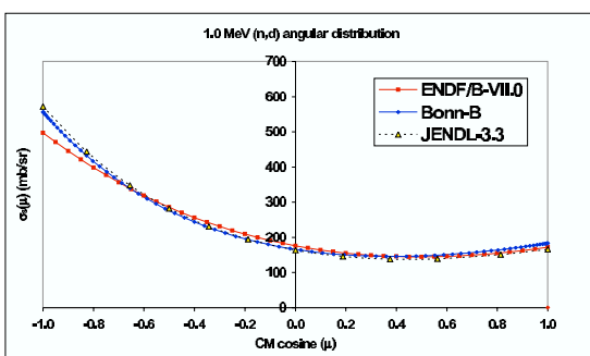
Fig. 6. As in figure 5 for 1.0 MeV neutrons.
