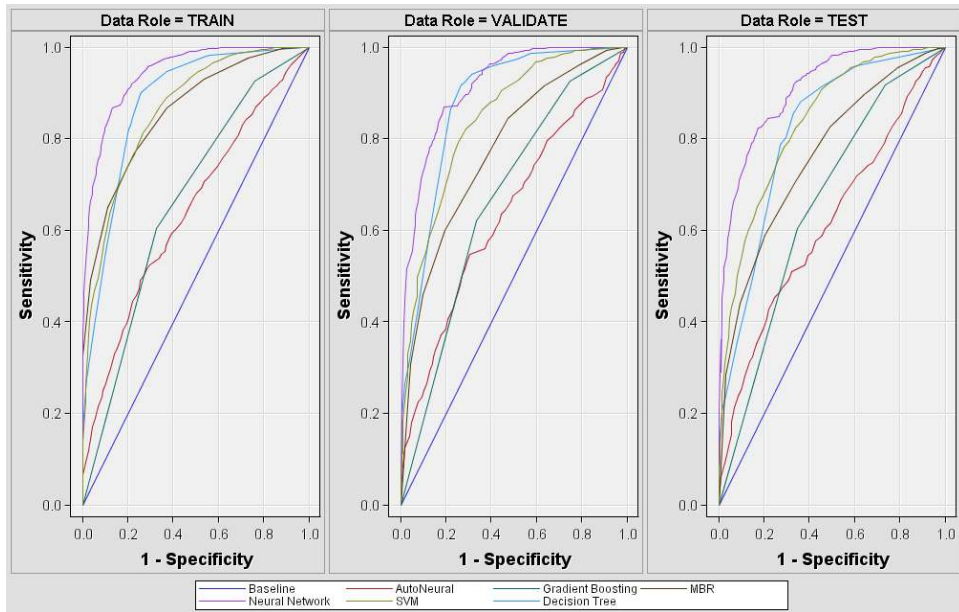
Figure 6: ROC Curves
