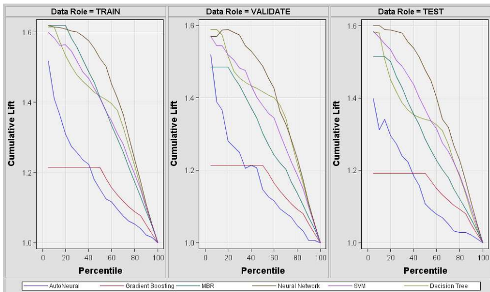
Figure 7: Cumulative Lift Plots
