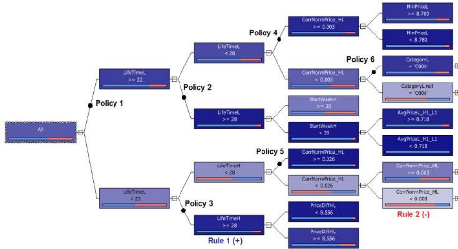
Figure 3: An Illustrative Decision Tree Model in Re-Mining
