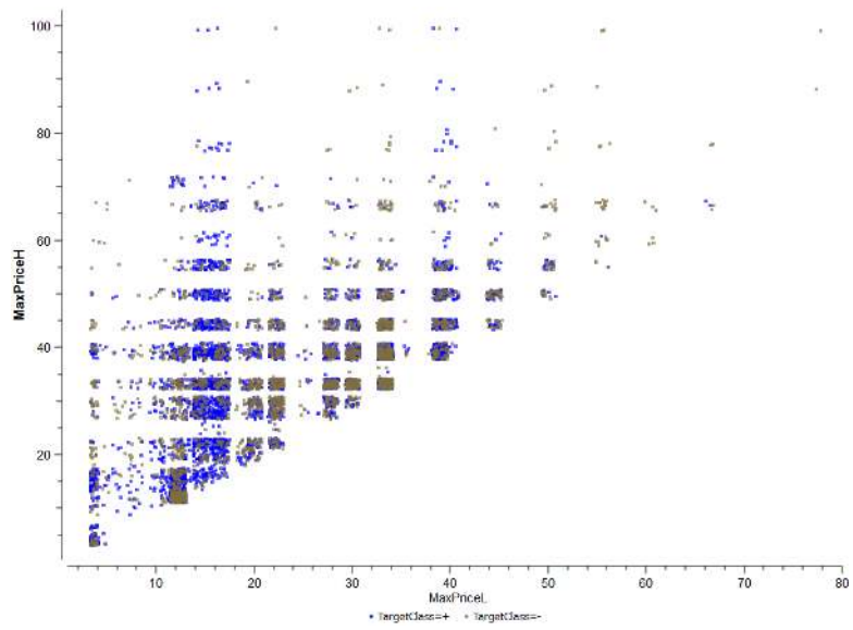
Figure 5: Exploratory Re-Mining Example: Effect of the Maximum Item Price
