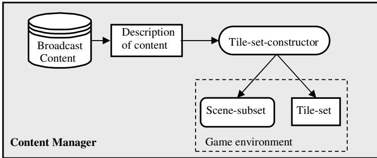
Figure 10: The content manager. Content description enables the tile-set-creator to select a scene-subset according to a chosen theme and to generate a legal tile-set from this subset. A legal-tile-set and the scene-subset form part of the game environment.
