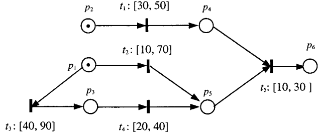
Fig. 2. Simple TPN model with concurrency, competence, and synchronization.
