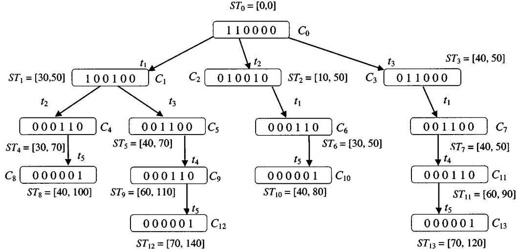
Fig. 3. Reachability tree of the TPN in Fig. 1.
