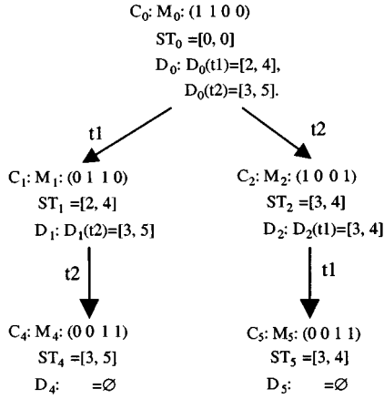
Fig. 4. Reachability tree of the TPN in Fig. 1 based on CS-state classes.
