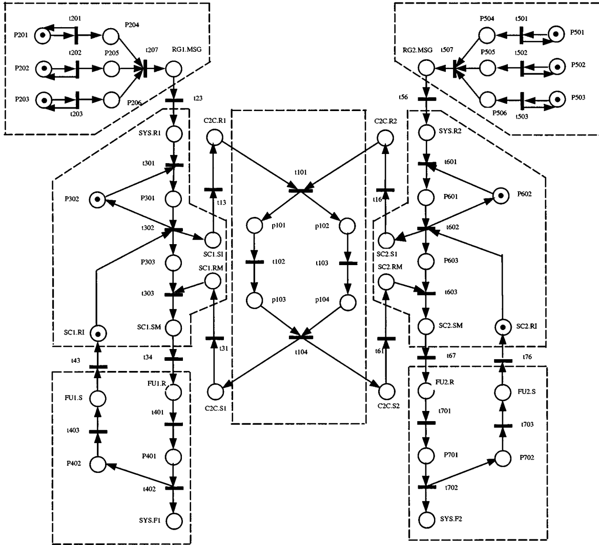
Fig. 7. TPN model of the C2 system.
