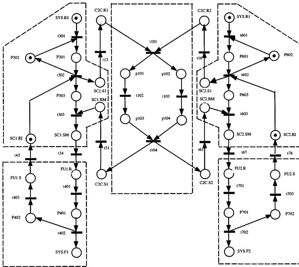
Fig. 8. Submodel for verifying requirement R1.
