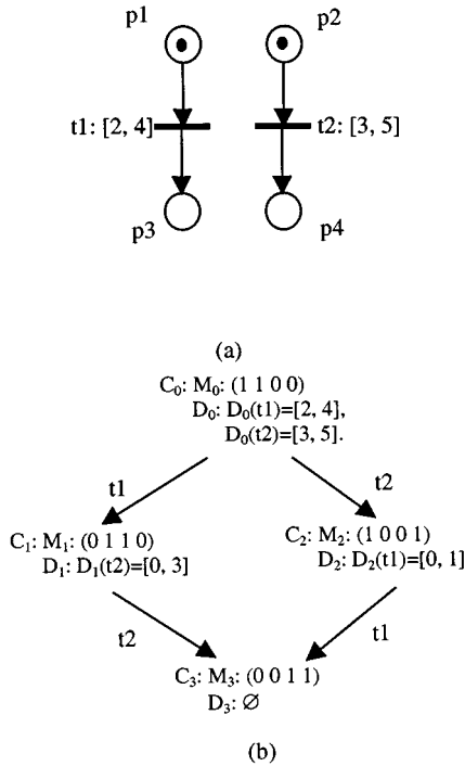
Fig. 1. (a) Simple TPN. (b) Reachability tree based on classic state classes.
