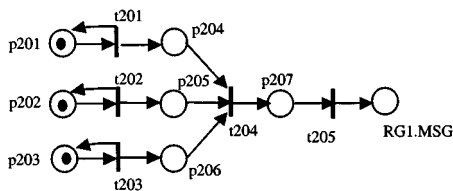
Fig. 11. Submodel for verifying requirement R4.
