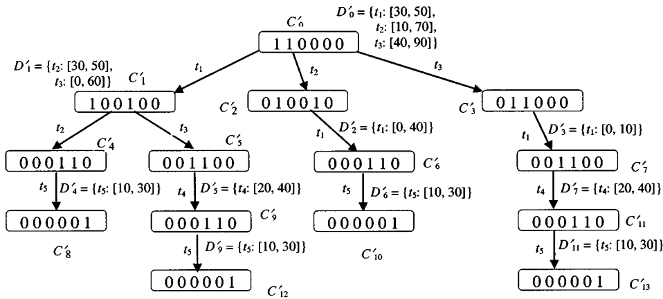
Fig. 5. Traditional reachability tree of the TPN in Fig. 2.
