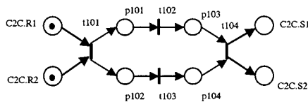
Fig. 10. Submodel for verifying requirement R3.
