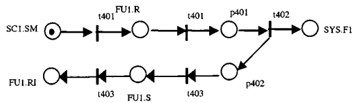
Fig. 9. Submodel for verifying requirement R2.
