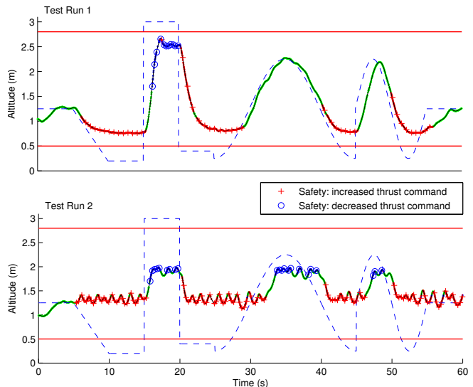
Fig. 3: Altitude trajectory of the quadrotor while learning the disturbance and tracking a reference. Run 1 is performed with a conservative disturbance model, while Run 2 is performed with an inferred model that fails to predict the true disturbance in certain regions of the state space.
