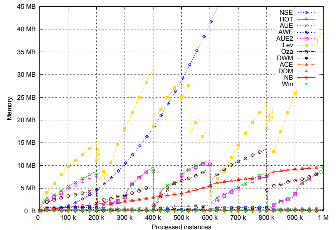
Fig. 3. Memory usage on the Tree_S dataset
