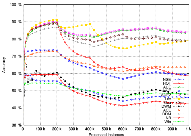
Fig. 2. Classification accuracy on the Tree_S dataset
