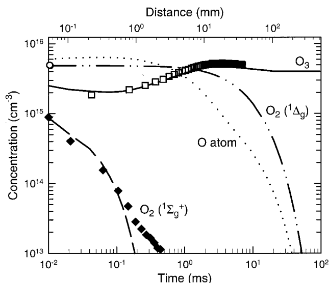
Figure 5. The dependence of the O, O 2 ( 1 Δ g ), O 2 ( 1 Σ g + ), and O 3 concentrations on time and distance for initial plasma operation at 24.4 W/cm 3 , 6.0 Torr of O 2 , and 120 °C (symbols are the experimental data, whereas the lines are the model prediction).
