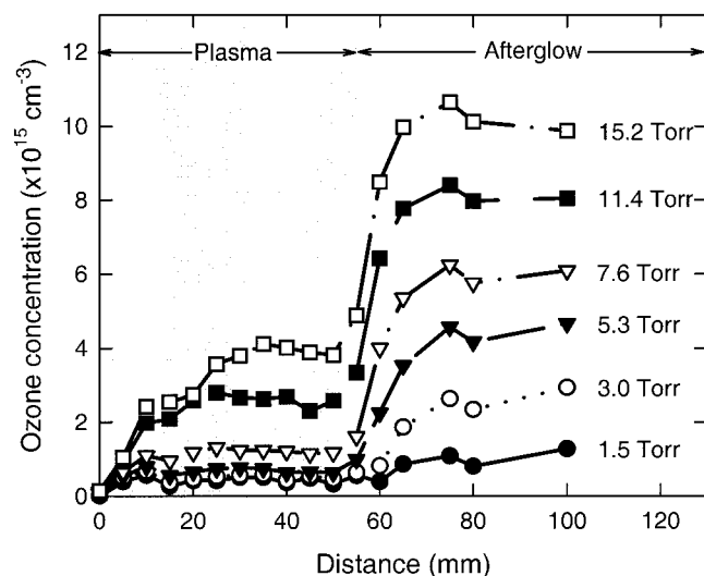
Figure 4. The dependence of the ozone concentration on axial position and oxygen partial pressure for an applied power of 24.4 W/cm 3 and a gas temperature of 120 °C.
