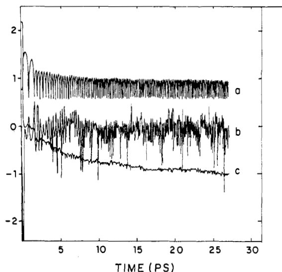
Figure 8. Excitation and recombination dynamics of 10 K \text{Br}_2\text{Ar}_{70} cluster excited to the {}^1\Pi_{1u} state: (a) \text{Br}_2 bond distance, (b) f_{\text{bond}} , (c) \text{Br}_2 bond energy. Units as in Figure 4.
