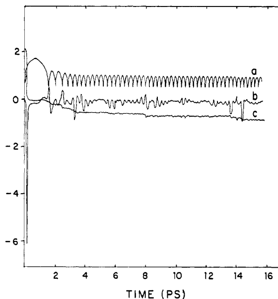
Figure 4. Excitation and recombination dynamics of 10 K \text{Br}_2\text{Ar}_{20} cluster excited to the repulsive ^1\Pi_{1u} state: (a) \text{Br}_2 bond distance in \sigma units vs. time (picoseconds); (b) force projection f_{\text{bond}} as defined in eq 6 in Verlet units; 22 (c) \text{Br}_2 bond energy in Verlet units (unit = 48 \epsilon or bromine X state D_e = 4.017 units).
