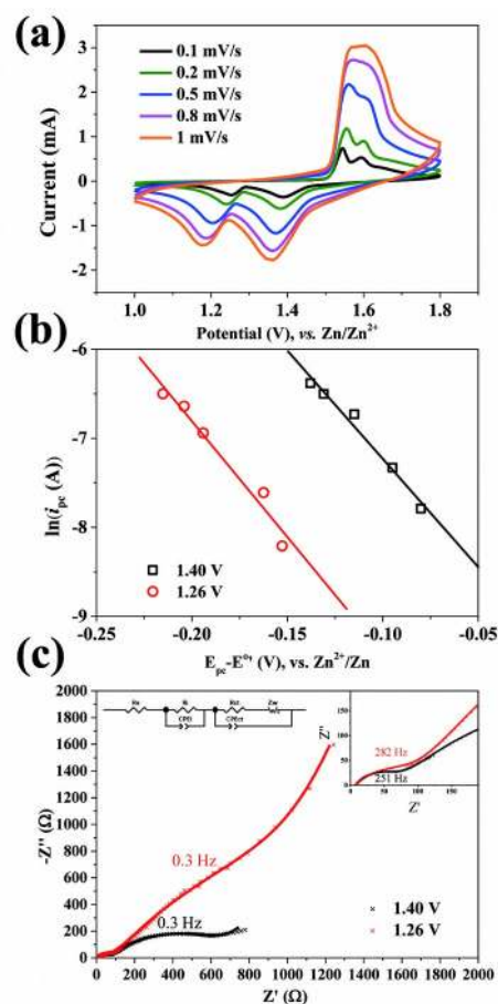
Fig. 6 (a) Cyclic voltammograms of in-situ deposited MnO 2 cathode at various scan rates (0.1, 0.2, 0.5, 0.8, 1.0 mV s -1 ). (b) Plots of ln i pc vs. ( E pc - E 0 ) for the 1.40 V and 1.26 V reductions. (c) EIS analysis of MnO 2 cathode discharged to 1.40 V and 1.26 V.
