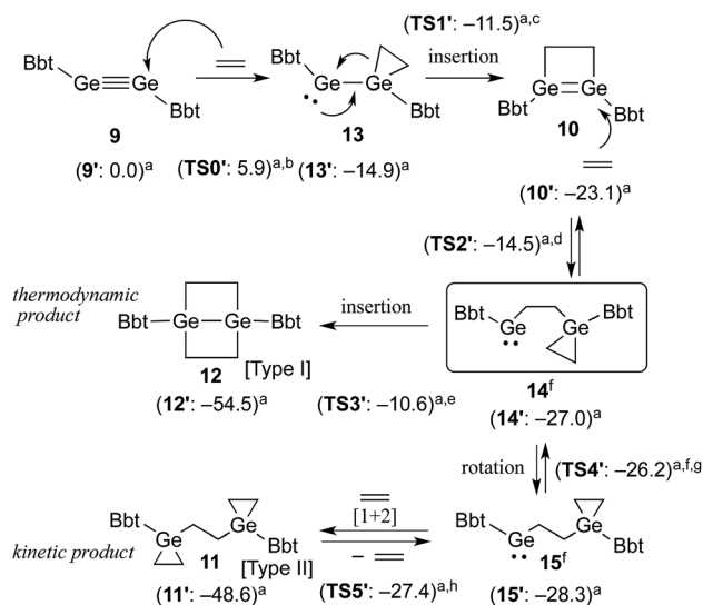
Scheme 3 Proposed mechanism for the reaction of 9 with ethylene. (a) Calculated relative energies (kcal mol -1 ) for model compounds bearing 2,6-[CH(SiMe 3 ) 2 ]-C 6 H 3 (Bbp) groups instead of Bbt groups. (b) \Delta E^\ddagger ( 9 – 13' ) = 5.9 kcal mol -1 . (c) \Delta E^\ddagger ( 13' – 10' ) = 3.4 kcal mol -1 . (d) \Delta E^\ddagger ( 10' – 14' ) = 8.6 kcal mol -1 . (e) \Delta E^\ddagger ( 14' – 12' ) = 16.4 kcal mol -1 . (f) 14 and 15 are rotational isomers with respect to a rotation around the central \text{GeH}_2\text{C}-\text{CH}_2\text{Ge} bond. (g) \Delta E^\ddagger ( 14' – 15' ) = 0.8 kcal mol -1 . (h) \Delta E^\ddagger ( 15' – 11' ) = 0.9 kcal mol -1 .
