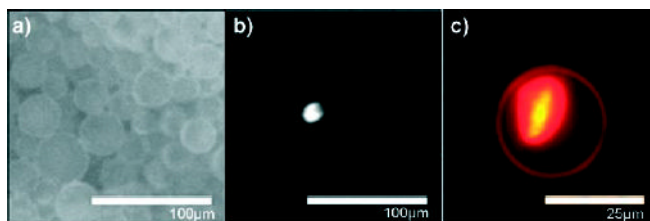
Figure 21. Fluorescence microscopy of a) GFP encapsulated in DOPC vesicles; b) a single HeLa cervical carcinoma cell (diameter 10 \mu\text{m} ) encapsulated in a DOPC vesicle; c) MCF7 breast cancer cell encapsulated in a DMPC vesicle. Reprinted from reference [177]. Copyright 2006 American Chemical Society. DOPC = dioleoylphosphatidylcholine, DMPC = dimyristoylphosphatidylcholine.
