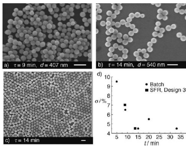
Figure 29. Synthesis of monodisperse particles of silica gel with a segmented-flow reactor (SFR). [192] Various residence times \tau resulted in silica particles with different average diameters d_{avg} . SEM microphotographs are shown for a) \tau = 9 min, d_{avg} = 407 nm, and b) \tau = 14 min, d_{avg} = 540 nm. c) Low-magnification SEM image of sample shown in (b). d) Standard deviation of the mean diameter \sigma versus \tau for particles formed by using an SFR or a batch reactor. Reprinted with permission from reference [192]. Copyright 2004 American Chemical Society.
