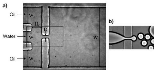
Figure 5. Formation of droplets by flow-focusing. [111] Modified from reference [111]. a) A schematic of the device. The rectangle outlines the field of view in (b). Copyright 2003 American Institute of Physics.
