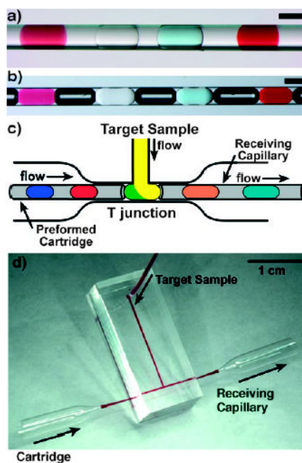
Figure 6. Preformed cartridges of plugs enable the combination of a large number of reagents with a sample in sub-microliter volumes. [42, 124] a,b) Four different reagents stored as an array of plugs in a capillary. The plugs are separated by a fluorocarbon carrier fluid, as well as air bubbles (in b), to prevent cross-communication between the plugs. Scale bars: 200 \mu\text{m} . c) Merging of plugs from a preformed cartridge with a target sample stream through a T junction. The resulting array of plugs is transferred into a receiving capillary and the trials are collected. d) Photograph of the T junction. Reprinted from reference [42] (a,b) and with permission from Elsevier from reference [124] (c,d).
