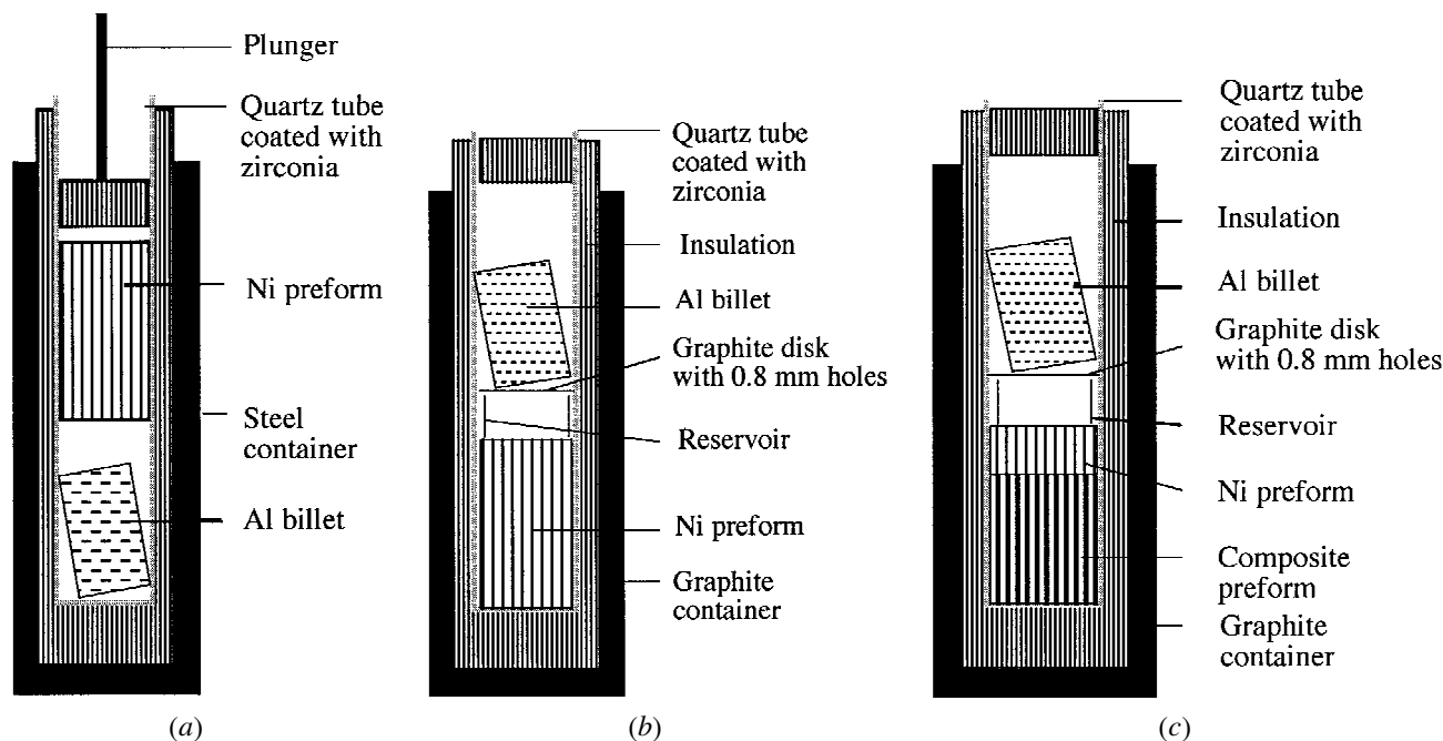
Fig. 1—Schematics illustrating processing of (1) NiAl from nickel-wire preforms using (a) a plunger and (b) gas pressure mechanisms; and (2) NiAl-composites (c) with tungsten.
