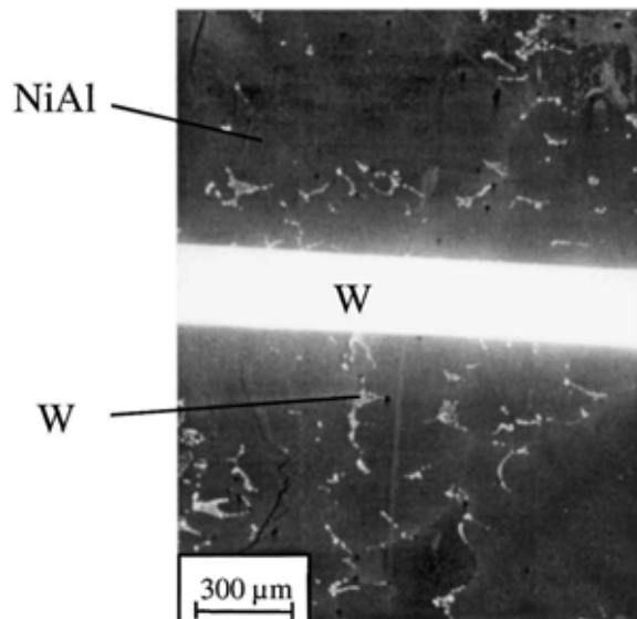
Fig. 3—SEM microstructure of a NiAl composite with 9 vol. pct tungsten obtained from an ingot with an average composition of 45 at. pct Ni, 46 at. pct Al, and 9 at. pct W (calculated based on the amounts of reactants, nickel and aluminum, present prior to reaction to form nickel aluminide).
