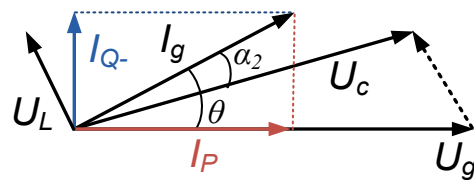
(b) Generate underexcited reactive power to converter ( I_{Q-} ).
