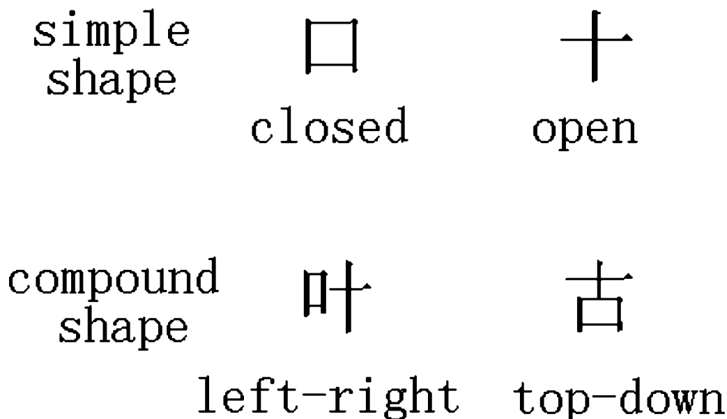
Figure 4. Illustration of visual requirements of Chinese characters. For simple characters (top), the global shape can be distinctive. For compound characters (bottom), the spatial relations between radicals are important. Both cases may be especially suited for visual areas that respond to low spatial frequency information.
