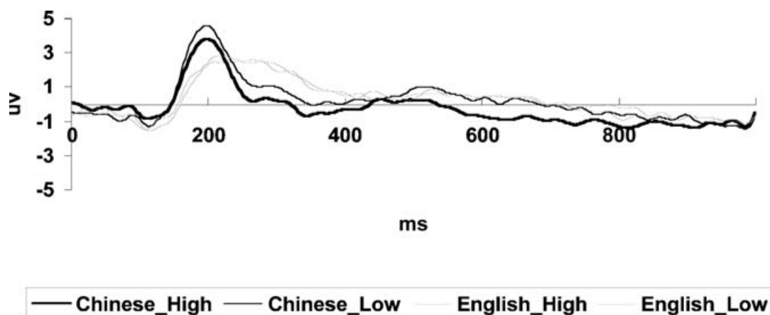
Figure 2. ERP bilingual results: waveform (at electrode Cz) from the onset of the target word read by Chinese–English bilinguals. Note that native language words, Chinese characters, produced an earlier peak of higher amplitude at 200 ms, compared with English words. Based on Liu and Perfetti, 2003.
