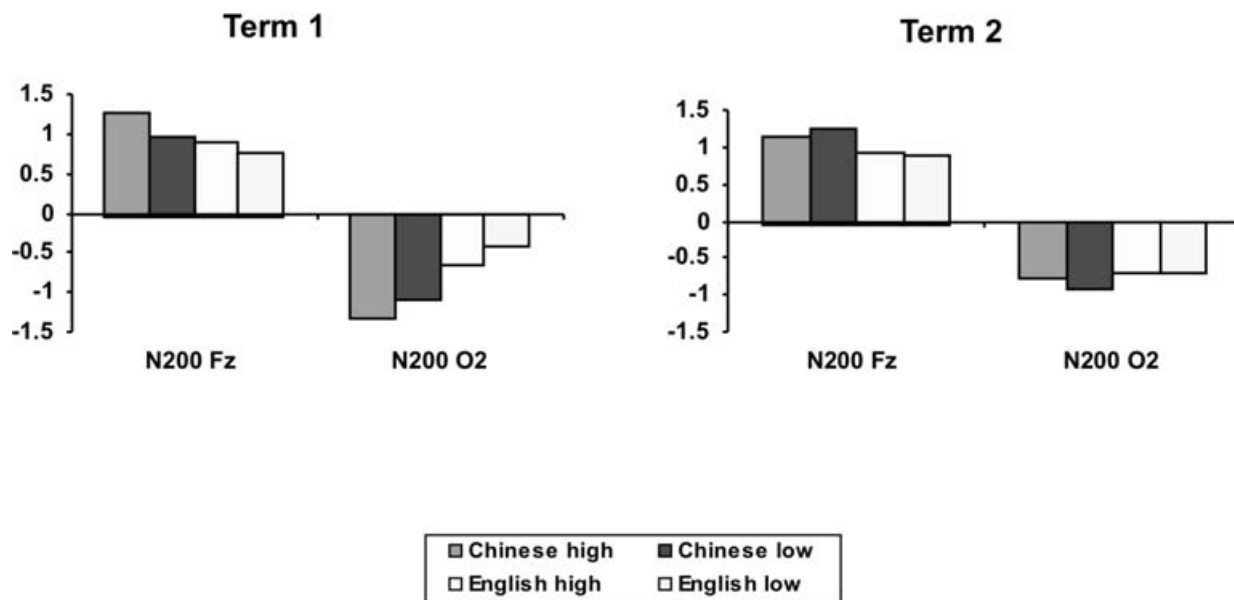
Figure 3. ERP Learning results: component scores from PCA analyses at two electrodes, frontal central (Fz) and right occipital (O2), at 200 ms. During the first term of learning Chinese, Chinese characters evoke differential responses for Chinese and English and for high vs. low frequency characters that are attenuated at term 2. Note for example, the high negativities for Chinese at the right occipital electrode at term 1 and their reduction at term 2. Chinese frequency effects disappear at term 2 across both sites. Based on Liu, Perfetti and Wang, 2006.
