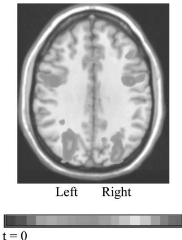
Figure 6. Comparison of laboratory learners showing activation in both left and right middle frontal areas for Chinese, relative to baseline. Horizontal view is at z = 33 . Peak activations for learned Chinese characters relative to baseline are left hemisphere (LH) -49, 12, 33 and right hemisphere (RH) 44, 14, 33 (Talairach). Adapted from Liu, Dunlap et al., in press.
