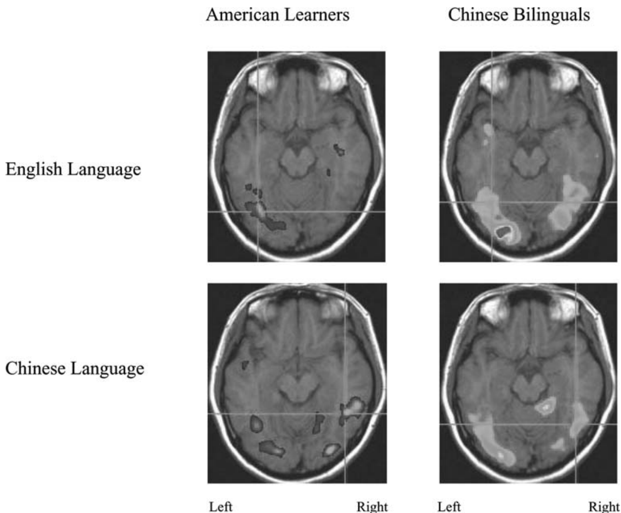
Figure 5. Horizontal views showing comparisons of classroom learners and native Chinese reading Chinese and English. Learners show a bilateral occipital and fusiform “Chinese” pattern for Chinese and a standard alphabetic pattern for English. Chinese natives show a Chinese pattern for both English and Chinese. Talairach coordinates for peak voxel activations are as follows. English learners of Chinese: English stimuli -35, -65, -12 ; Chinese stimuli -43, -44, -9 ; Chinese bilinguals: English stimuli -33, -56, -12 ; Chinese stimuli -43, -54, -12 . Based on Nelson et al., 2005.
