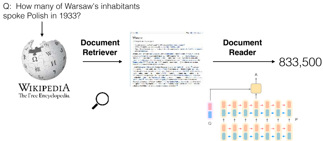
Figure 1: An overview of our question answering system DrQA.
