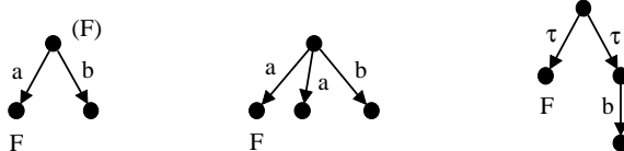
Figure 2: Backward propagation of inconsistencies.
