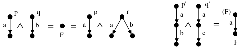
Figure 1: Basic intuition behind conjunctive composition.
