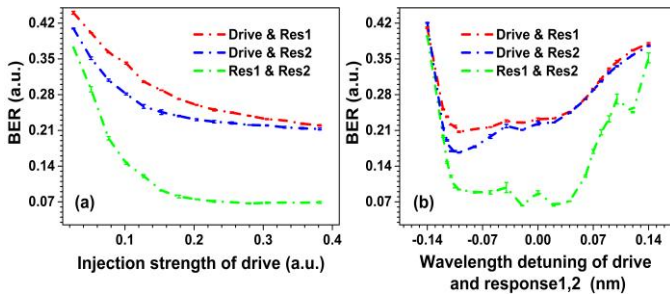
Fig. 6. BERs between drive, response1,2 as a function of (a) injection strength of drive, (b) wavelength detuning of drive and response1,2.
