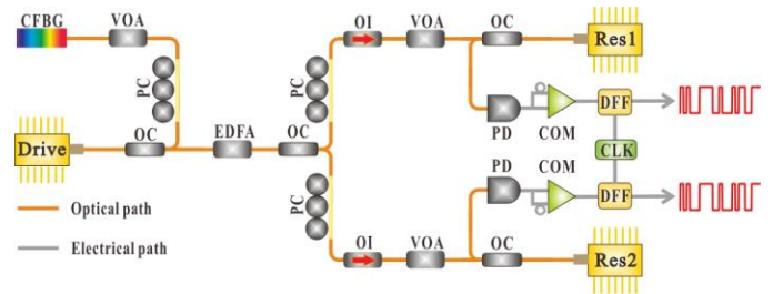
Fig. 1. Experimental setup. Drive: drive laser, Res1,2: response lasers, CFBG: chirped fiber Bragg grating, OC: optical coupler, PC: polarization controller, VOA: variable optical attenuator, EDFA: erbium-doped fiber amplifier, OI: optical isolator, PD: photodetector, COM: one-bit differential comparator, DFF: D-type flip-flop, CLK: trigger clock.
