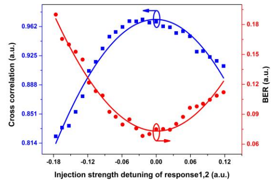
Fig. 7. Cross correlation and BER of the response lasers a function of the injection strength detuning between them.
