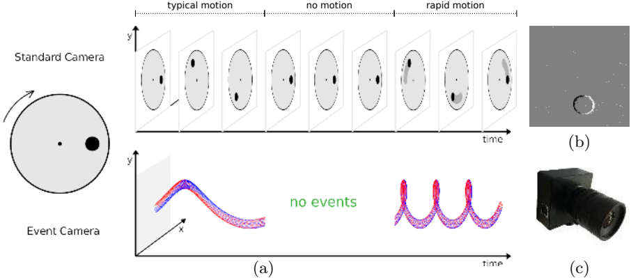
Fig. 1. Event-based camera: (a): in contrast to standard video frames shown in the upper graph, a stream of events from an event camera, plotted in the lower graph, offers no redundant data output, only informative pixels or no events at all. Red and blue dots represent positive and negative events respectively (this figure was recreated inspired by the associated animation of [19]: https://youtu.be/LauQ6LWTkxM?t=35s ). (b): image-like visualisation by accumulating events within a time interval — white and black pixels represent positive and negative events respectively. (c): the first commercial event camera, DVS128, from iniLabs Ltd.
