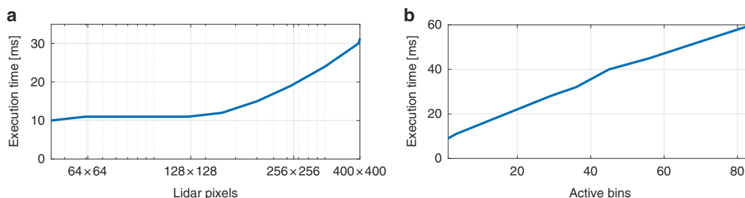
Fig. 5 Execution time of the proposed method. The execution time is shown as function of a lidar pixels (having a mean of 4 active bins per pixel), and b histogram bins with non-zero counts, for an array of 141 \times 141 pixels. As all the steps involved in the reconstruction algorithm can process the pixel information in parallel, the total execution time does not increase significantly when more pixels are considered. However, as the pixel-wise operations are not fully parallel, there is a linear dependency on the number of active (non-zero) bins present in the lidar frame
