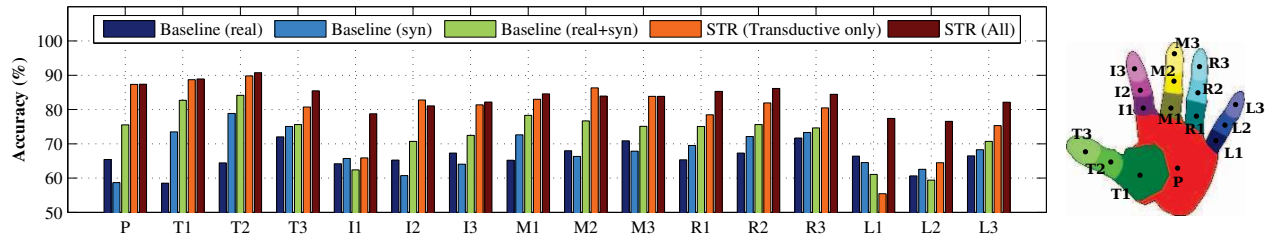
Figure 4: Joint classification accuracy of the single view sequence.
