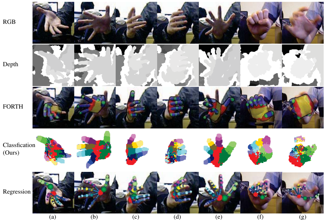
Figure 6: Qualitative results of the multi-view experiment. (a)-(e) are taken from sequence B and (f)-(g) are from sequence C . Hand regions are cropped from the originals for better visualisation ( 135 \times 135 pixels for (a)-(e), 165 \times 165 pixels for (f)-(g)). The resolution of the original images are 640 \times 480 . Joint labels follow the color scheme in Figure 4.
