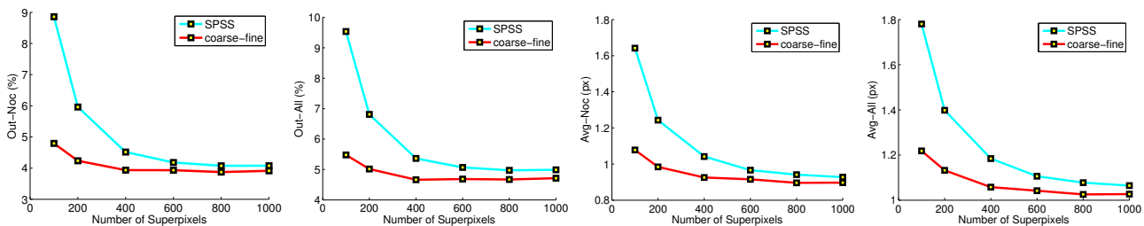
Figure 8. Performance as a function of number of superpixels on KITTI : comparison with [31] after running both algorithms for 1 iteration.
