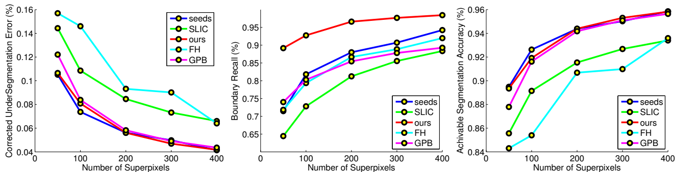
Figure 4. BSD : In this experiment we use the position weight to be 0 for both our approach and SLIC to mimic SEEDS that does not use regularization. Note that our approach outperforms both baselines. Speed: SEEDS( 30Hz), SLIC( 5HZ), OURS( 30HZ)
