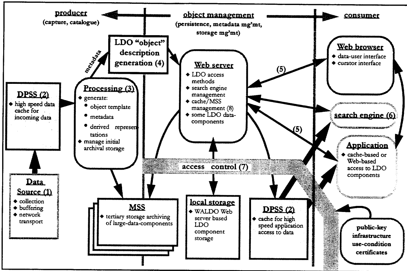
Figure 8. The distributed Large-Data-Object overall architecture and data flow.
