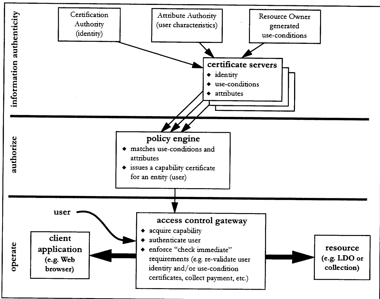
Figure 14. The Use-Condition based Security Architecture.
