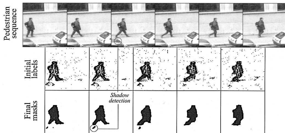
Fig. 10. Mask quality.
