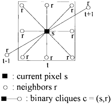
Fig. 1. Spatiotemporal neighborhood and binary cliques.
