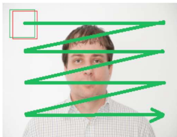
Figure 2: Face detection scans each image frame; in practice the entire image frame does not need to be scanned if a-priori data can be used to predict where the face will be found in the current frame.
