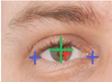
Figure 5: Key points within the eye-socket region; the eye corners (blue crosses); the pupil center (large green cross); and the estimated center of the eye-socket region (red cross).
