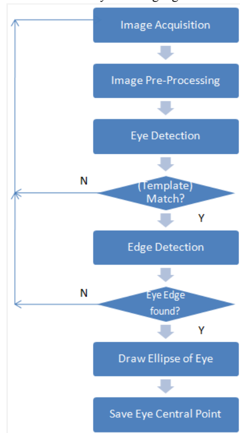
Figure 1. Flowchart of the Real-time Eye Tracking Algorithm
