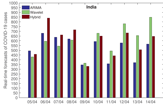
Fig. 4. Figures of (a) Actual Vs. predicted (Hybrid ARIMA-WBF Model) values for India COVID-19 data; (b) Real-time forecasts (10 days) of the number of cases for India.
