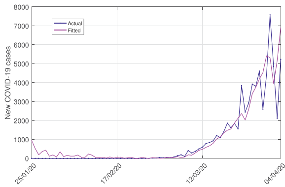
Fig. 3. Figures of (a) Actual Vs. predicted (Hybrid ARIMA-WBF Model) values for France COVID-19 data; (b) Real-time forecasts (10 days) of the number of cases for France.
