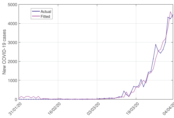
Fig. 6. Figures of (a) Actual Vs. predicted (Hybrid ARIMA-WBF Model) values for the UK COVID-19 data; (b) Real-time forecasts (10 days) of the number of cases for the UK.
