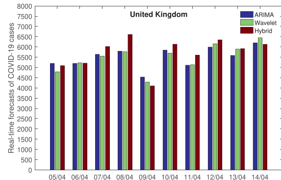
Fig. 6. Figures of (a) Actual Vs. predicted (Hybrid ARIMA-WBF Model) values for the UK COVID-19 data; (b) Real-time forecasts (10 days) of the number of cases for the UK.
