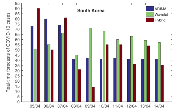
Fig. 5. Figures of (a) Actual Vs. predicted (Hybrid ARIMA-WBF Model) values for South Korea COVID-19 data; (b) Real-time forecasts (10 days) of the number of cases for South Korea.
