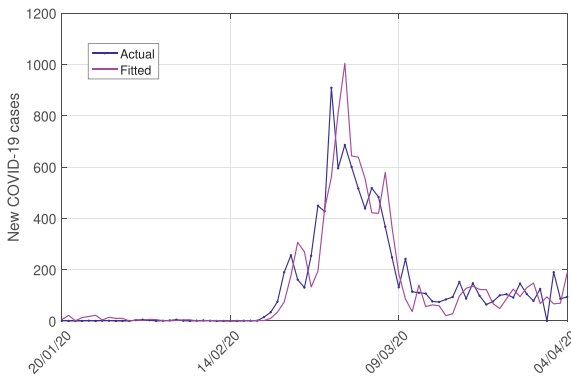
Fig. 5. Figures of (a) Actual Vs. predicted (Hybrid ARIMA-WBF Model) values for South Korea COVID-19 data; (b) Real-time forecasts (10 days) of the number of cases for South Korea.
