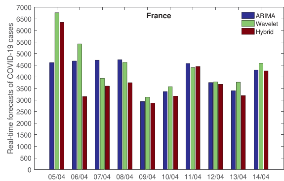
Fig. 3. Figures of (a) Actual Vs. predicted (Hybrid ARIMA-WBF Model) values for France COVID-19 data; (b) Real-time forecasts (10 days) of the number of cases for France.
