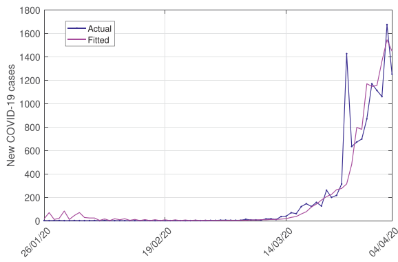
Fig. 2. Figures of (a) Actual Vs. predicted (Hybrid ARIMA-WBF Model) values for Canada COVID-19 data; (b) Real-time forecasts (10 days) of the number of cases for Canada.
