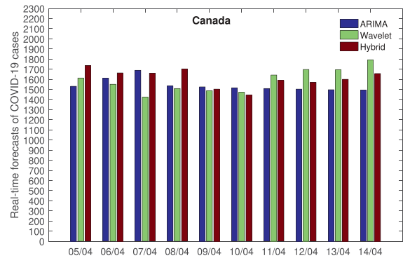
Fig. 2. Figures of (a) Actual Vs. predicted (Hybrid ARIMA-WBF Model) values for Canada COVID-19 data; (b) Real-time forecasts (10 days) of the number of cases for Canada.
