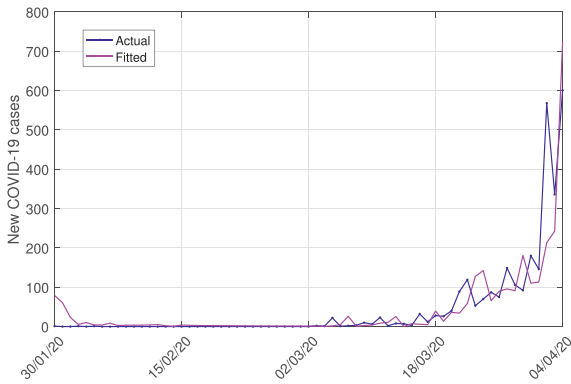
Fig. 4. Figures of (a) Actual Vs. predicted (Hybrid ARIMA-WBF Model) values for India COVID-19 data; (b) Real-time forecasts (10 days) of the number of cases for India.
