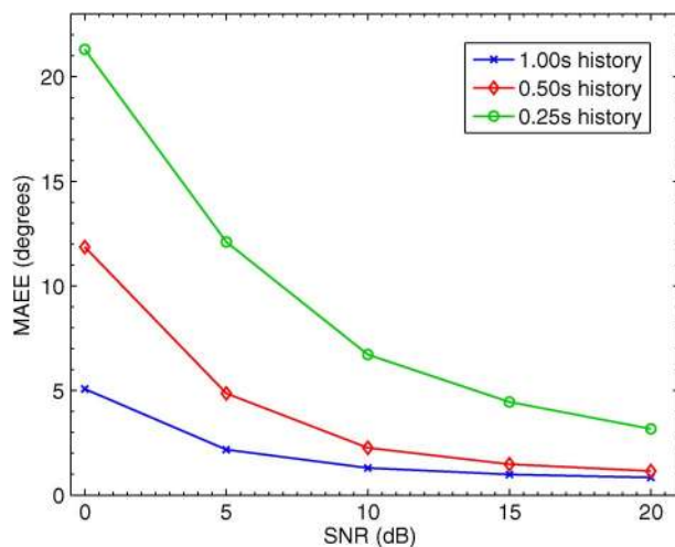
Fig. 9. DOA estimation error vs SNR for four intermittent speakers in a simulated reverberant environment.
