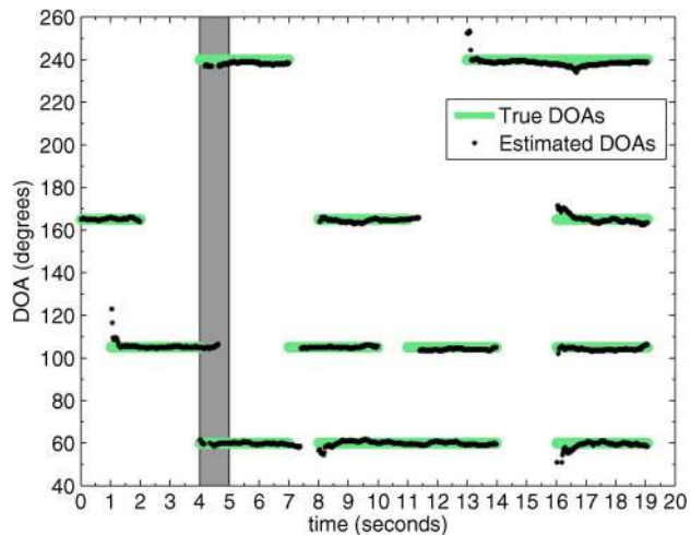
Fig. 8. Estimation of DOA of four intermittent speakers at 60^\circ , 105^\circ , 165^\circ , and 240^\circ in a simulated reverberant environment with 20 dB SNR and a one-second block size. The gray-shaded area denotes an example “transition period.”
