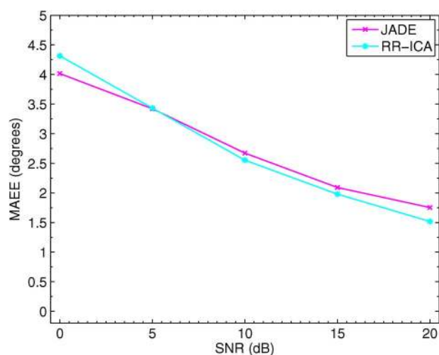
Fig. 15. DOA estimation error vs SNR for six static speakers in a simulated reverberant environment.
