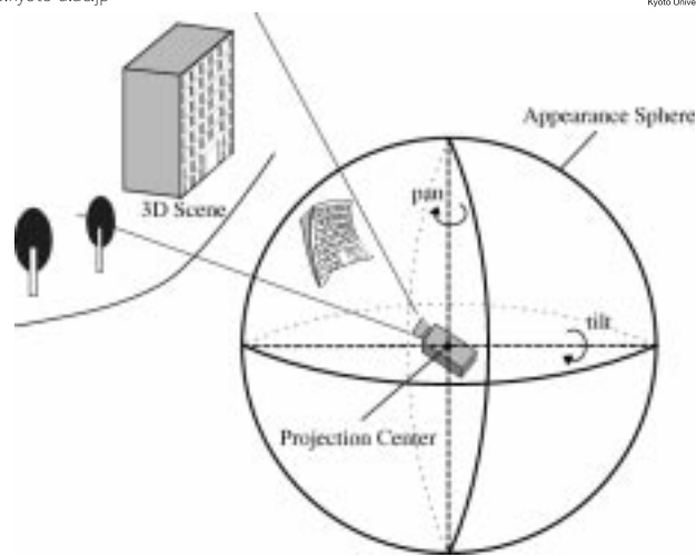
Fig. 2. Fixed-viewpoint pan-tilt camera.
