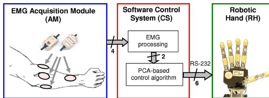
Figure 1 System overview. The experimental setup included the EMG acquisition module (AM, with four active electrodes placed on the user's forearm and an acquisition board) and the software control system (CS), which ran on a laptop and was interfaced with the hand (RH) via serial port. The CS acquired and decoded the four EMG signals to generate two independent input signals; these were fed into the PCA-based algorithm that generated and sent the six motor control commands to the robotic hand.
