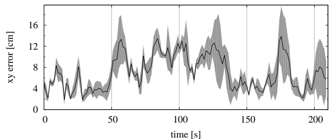
Fig. 5. Localization error as mean and standard deviation for five runs in scenario 1.
