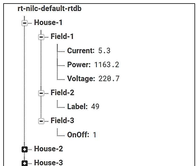
Figure 6. Process of Firebase real-time database.
