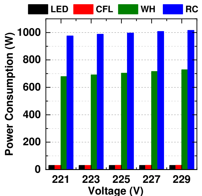
Figure 3. Power consumption of LED, CFL, rice cooker, and water heater with voltage change.
