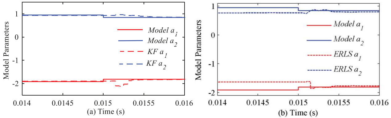
Fig. 13. Real-time parameters estimation during a step load change from 5 \Omega to 1 \Omega at 0.015s, (a) KF, (b) ERLS
