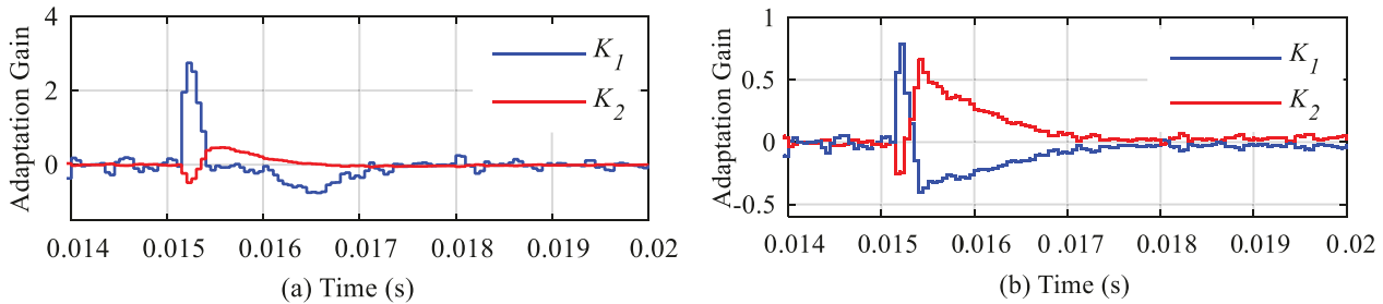
Fig. 14. Kalman Gains, (a) KF, (b) ERLS.
