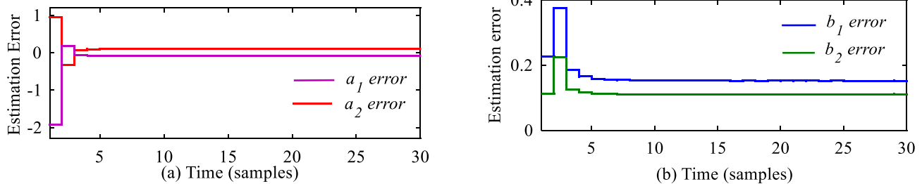
Fig. 9. The estimation error for ERLS during steady state operation. (a) Denominator coefficients. (b) Numerator coefficients.
