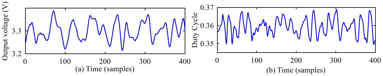
Fig. 7. Experimental filtered data sampled at 20 kHz (a) output voltage (zoom-in) (b) duty cycle
