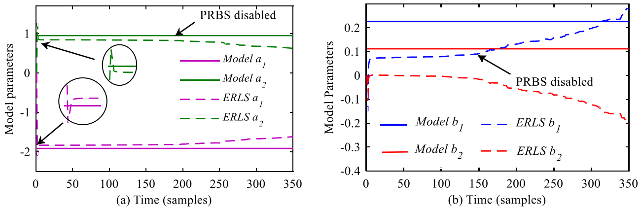
Fig. 8. The estimation results using ERLS with \lambda=0.95 . (a) Denominator coefficients. (b) Numerator coefficients.
