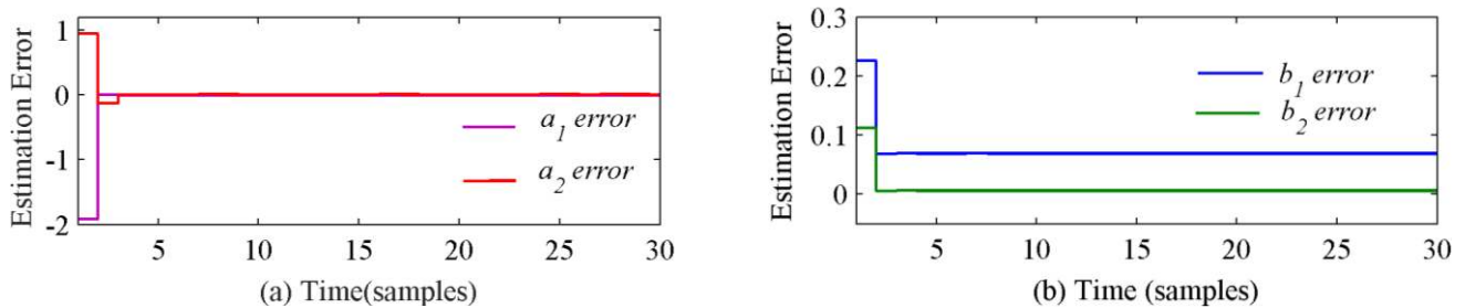
Fig. 11. The estimation error for KF during steady state operation. (a) Denominator coefficients. (b) Numerator coefficients
