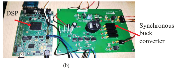
Fig. 5. Experimental setup of a synchronous buck converter for real-time parameter estimation. (a) Block diagram (b) Overview of test board.
