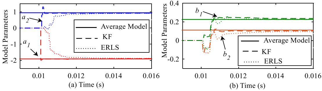
Fig. 2. On-line parameter estimation results using ERLS and KF. (a) Denominator coefficients. (b) Numerator coefficients.
