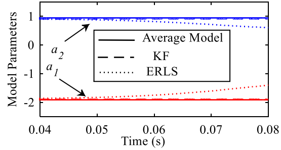
Fig. 4. Estimator wind-up effect on ERLS and KF.
