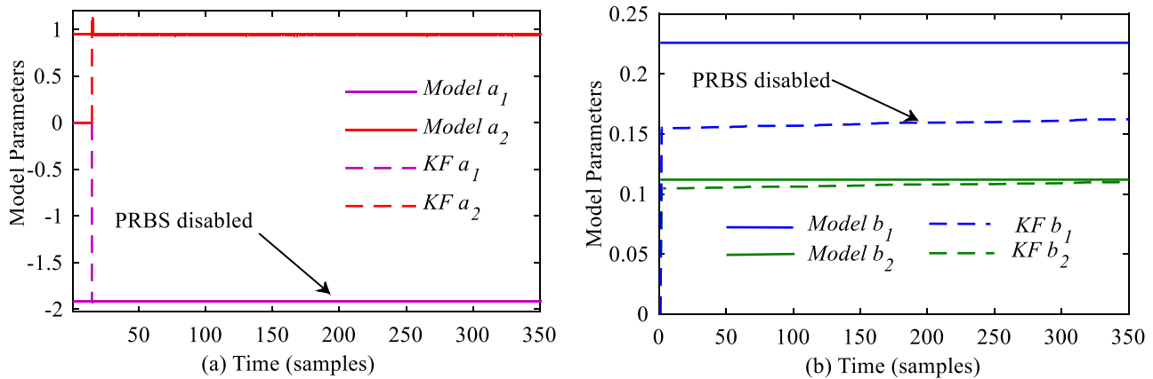
Fig. 10. The estimation results using KF. (a) Denominator coefficients. (b) Numerator coefficients.
