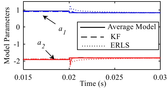
Fig. 3. On-line parameters estimation during a step load change from 5 Ω to 1 Ω at 0.02s for ERLS and KF
