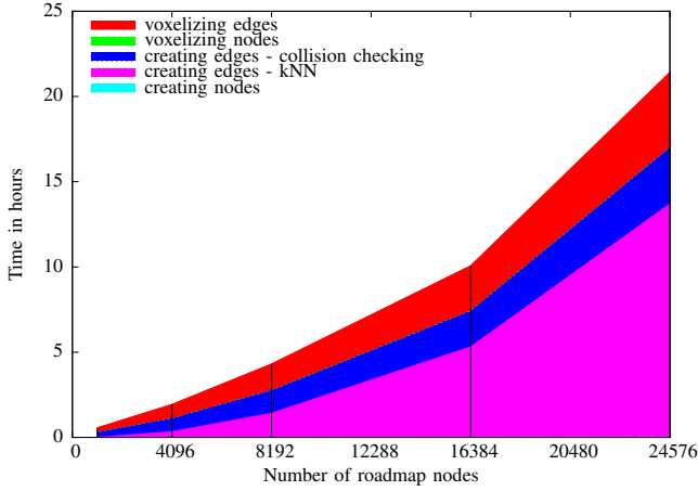
Fig. 4. Preprocessing time
