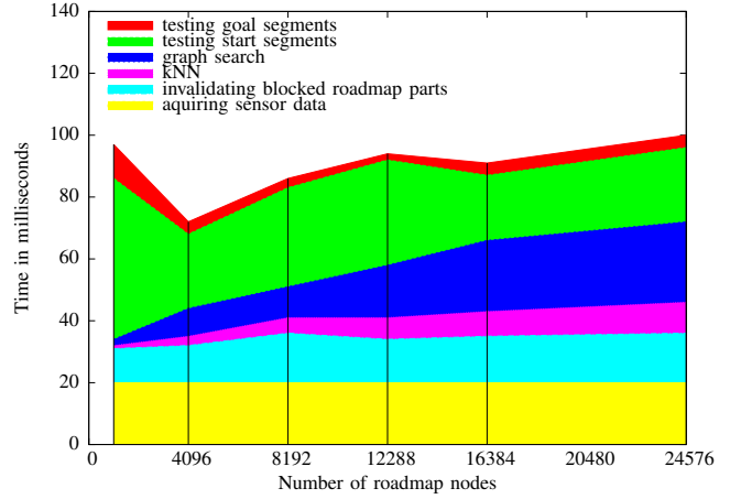
Fig. 5. Planning time
