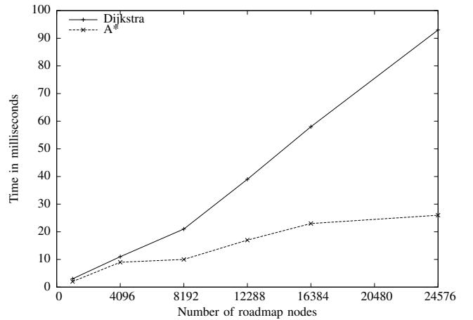
Fig. 6. Comparison of search times using A* and Dijkstra's algorithm
