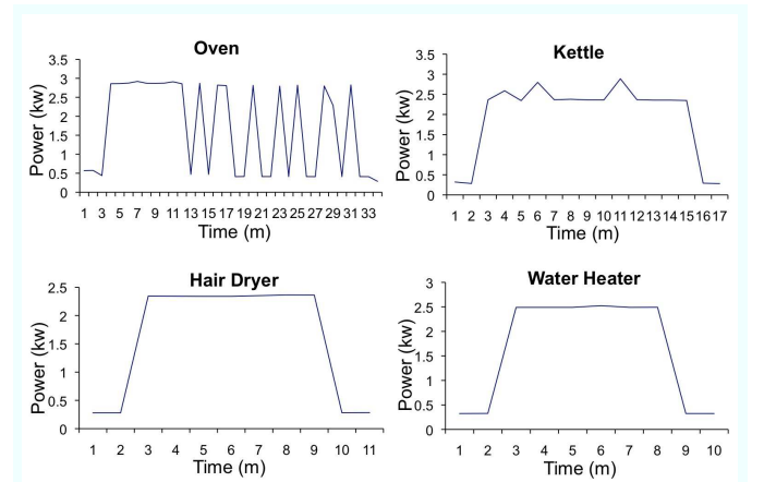
Fig. 4. Active Power Signatures for 4 appliances
