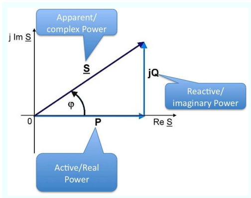
Fig. 3. Relation between reactive and active power
