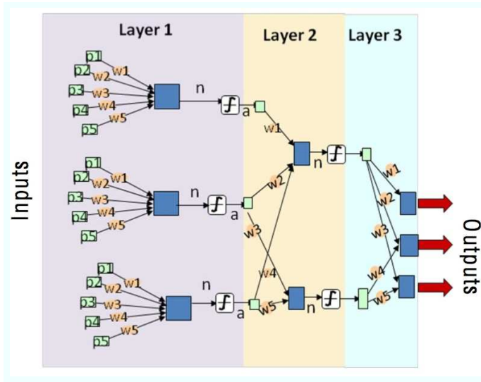
Fig. 7. An example of 3-layer ANN showing input, hidden and output neurons
