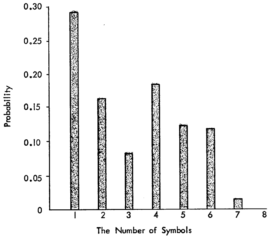
FIG. 5 - The Probability of a Number of Symbols Having the Same First Four Direction Segments.
