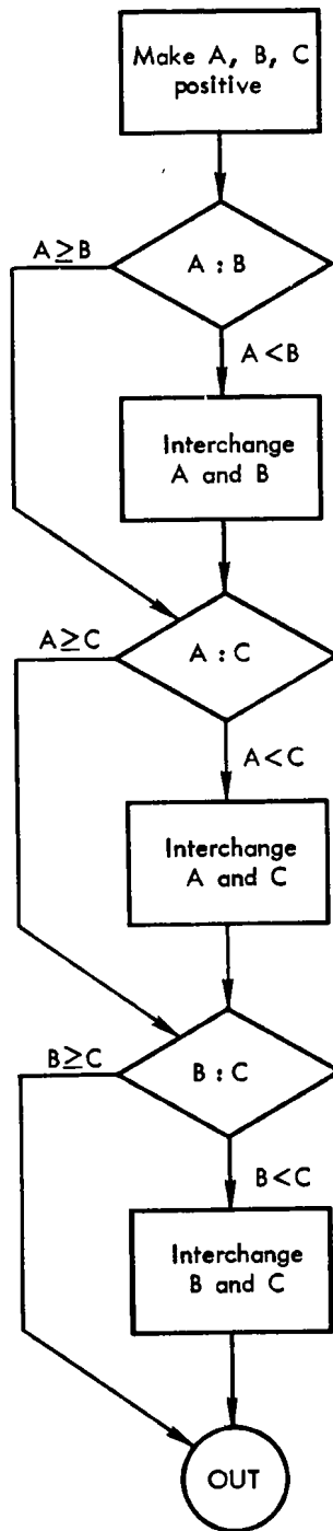
FIG. 8 (b) - Flowchart of Problem B Coded in the Experiment: A Method of Sorting Three Numbers into a Descending Sequence of Their Magnitudes.
