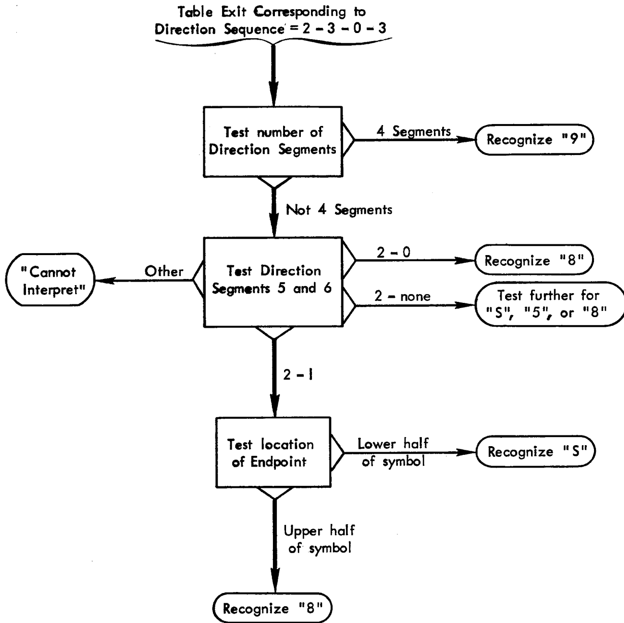
FIG. 6 - Recognition of the Track of Figure 2.
