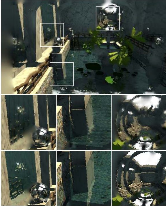
Figure 11: Top: Impact on the warping quality caused by JPEG-compressed depth. Bottom: Uncompressed depth.
