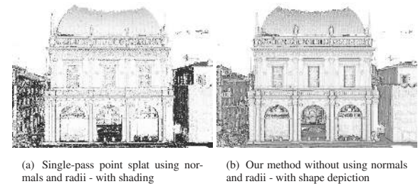
Figure 12: Loggia (110Mpts): (a) single-pass point splat with shading and (b) our method with shape depiction.
