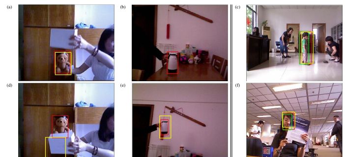
Figure 2: DS-KCF (red box) v. KCF (yellow box). Occlusion handling: (a) before occlusion, and (d) after occlusion. Change of scale: (b) initial target, and (e) target after change of scale. DS-KCF (red) v. Prin-Track(RGBD) (yellow) v. groundtruth (green) on (c) ‘child_no1’, and (f) ‘face_occ5’.
