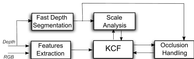
Figure 1: Block diagram of the proposed DS-KCF tracker.
