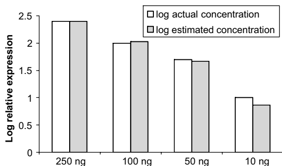
Figure 5 Comparison of the actual amount of RNA used in different reverse transcription reactions with the respective amount of HuPO cDNA measured by real time RT-PCR. There is good correlation between the RNA concentration used and the real time PCR estimation of the different amounts of HuPO cDNA (using omniscrypt reverse transcriptase).
