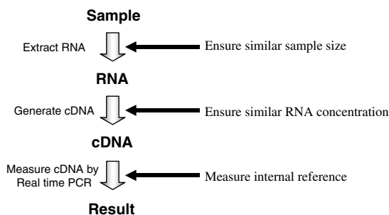
Figure 1 Processes required to generate a real time RT-PCR result. Black arrows indicate points, which should be considered for a good normalisation strategy.
