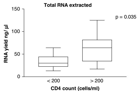
Figure 2 Total RNA yields from two different groups of HIV patients. Total RNA extracted using PAXtubes (Qiagen) as for Dheda et al. 5
