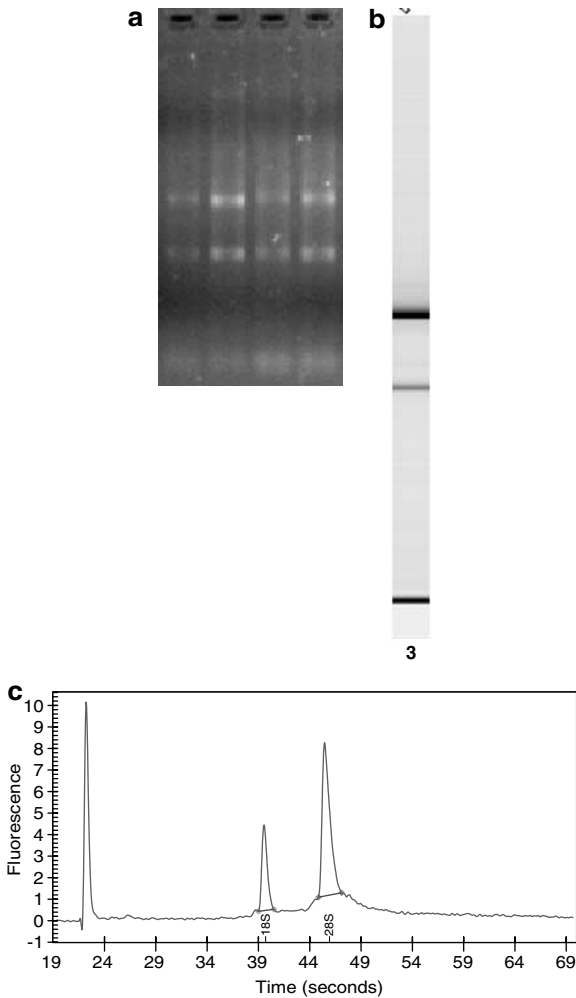
Figure 3 Example of good quality RNA assessed by (a) agarose gel (5 ml RNA extract), (b and c) by the Agilent Bioanalyser (1 ml RNA extract) using the RNA LabChip. Total RNA extracted using PAXtubes (Qiagen) as for Dheda et al . 5
