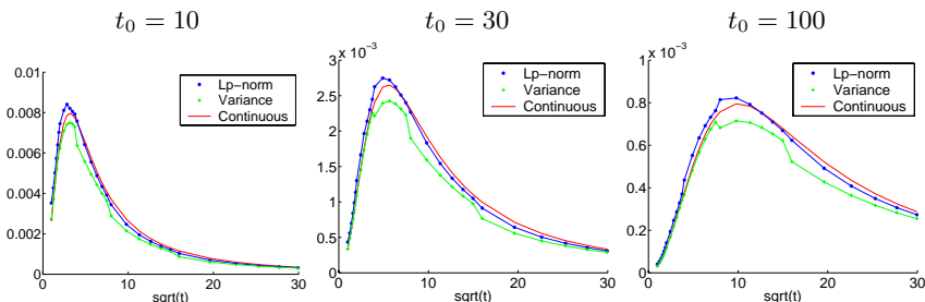
Fig. 3: Scale-space signatures of the (negative) normalized Laplacian response for rotationally symmetric Gaussian blobs with variances t_0 = 10 , t_0 = 30 and t_0 = 100 , respectively, computed using a separable BIN3(6)PYRAMID in two dimensions using l_p -normalization (stars) and variance-based normalization (crosses). For reference, the corresponding continuous behaviour is shown as well (solid curve).
