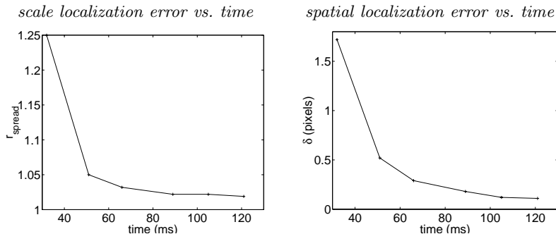
Fig. 4: Trade-offs between the localization error (vertical axis) and the computation time (horizontal axis) for hybrid pyramids with different values of \rho : (left) scale localization error, (right) spatial localization error.
