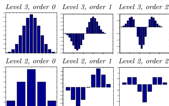
Fig. 2: Examples of equivalent convolution kernels and equivalent derivative approximation kernels for the BIN5PYRAMID derived from the BIN5REDUCECYCLE in figure 1.
