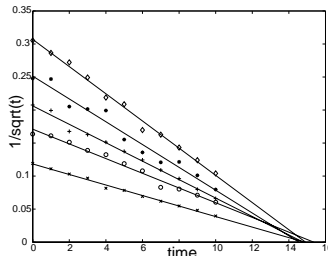
Fig. 6: Graph showing the variation over time of 1/\sqrt{t} for five image features matched over time as a camera approaches an object with uniform velocity.
