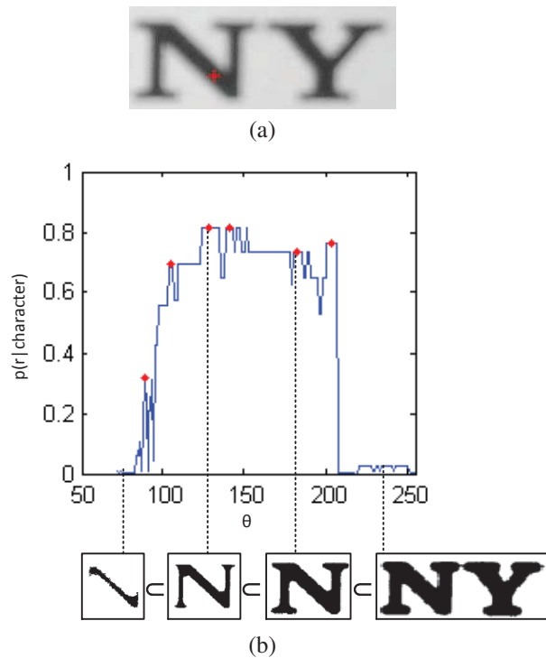
Figure 6. In the first stage of the sequential classification the probability p(r|\text{character}) of each ER is estimated using incrementally computable descriptors that exploit the inclusion relation of ERs. (a) A source image cut-out and the initial seed of the ER inclusion sequence (marked with a red cross). (b) The value of p(r|\text{character}) in the inclusion sequence, ERs passed to the second stage marked red
