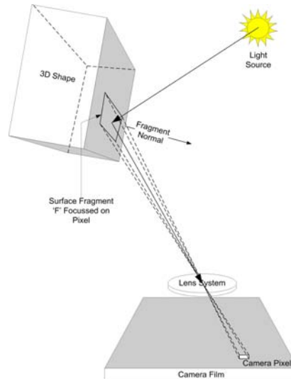
Figure 5. Fragment Pipeline's Camera Model
