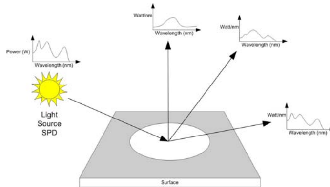
Figure 3. Spectral BRDF
