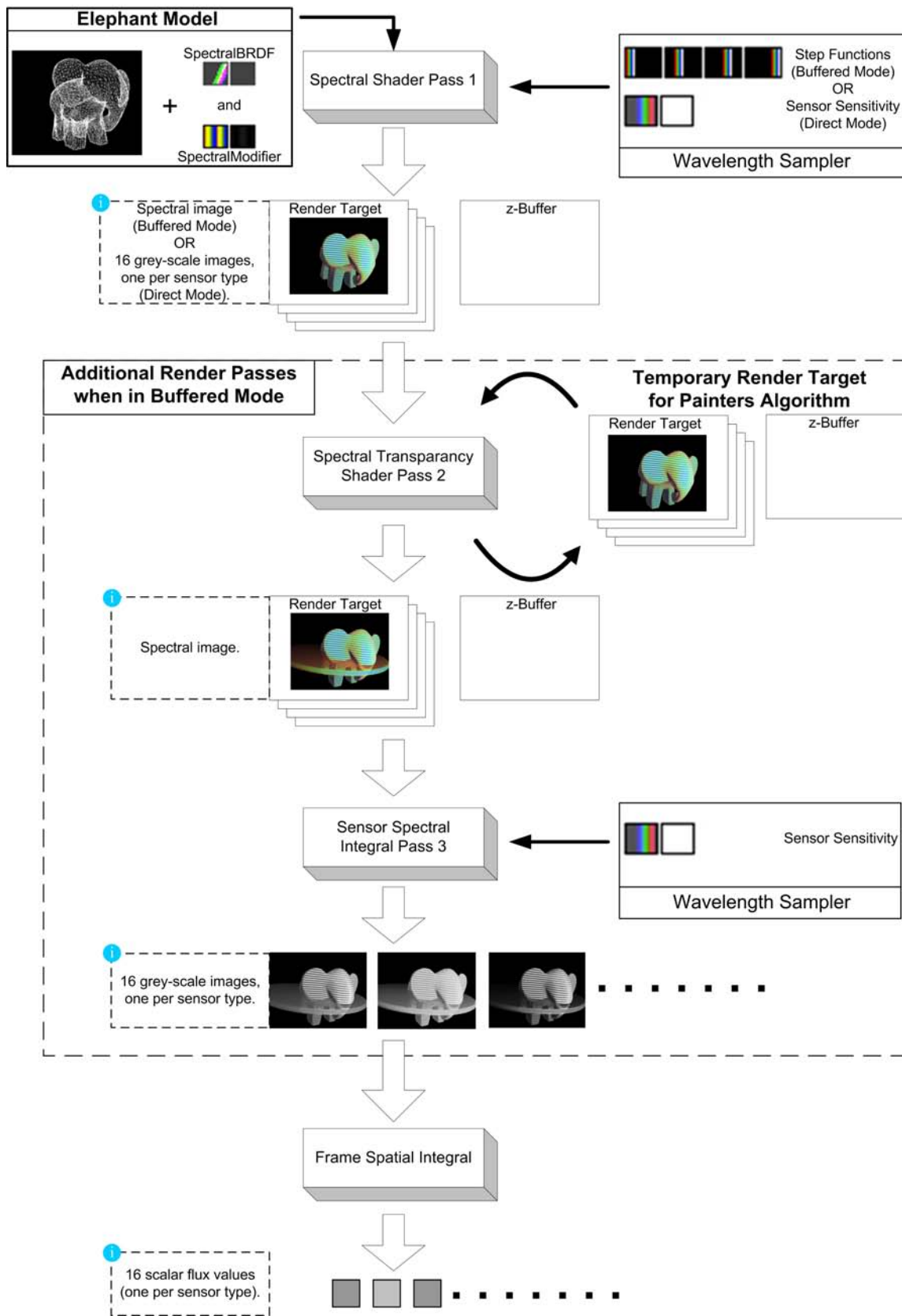
Figure 6. Expanded Fragment Processor
