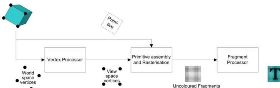
Figure 1. The historical Fixed Pipeline Computer Graphics System
