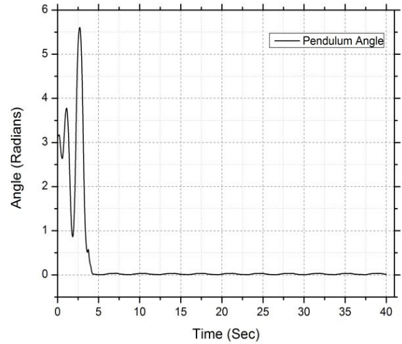
FIGURE 9. Pendulum angle for optimized FLC.
