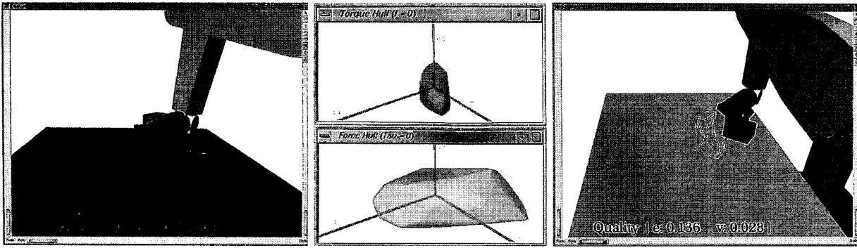
Figure 6: (Left) A stable grasp of the L-shaped object. The axes are positioned at the object's center of gravity (Z axis points into the table). (Middle Top) The 6D grasp wrench space projected into torque space by setting the net force to 0. (Z axis points up). (Middle Bottom) The GWS projected into force space by setting the net torque to 0. (Right) The task is planned in GrasPlt by moving the object from its original location (empty wireframe) to its destination point and saving the new object pose.
