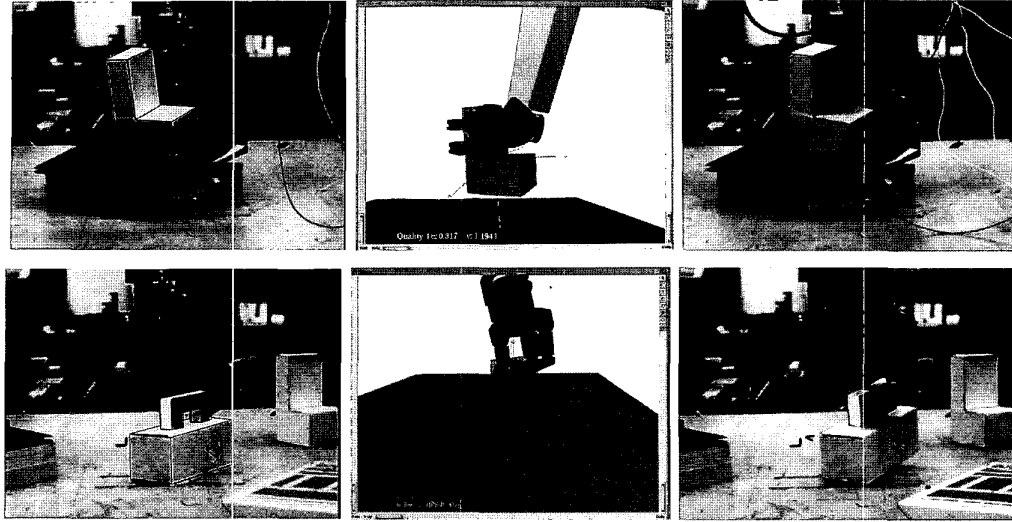
Figure 5: [Row 1] Left: The vision system determines the pose of the L-shaped object within the robot workspace. Middle: A stable grasp planned within GraspIt. Right: The completed grasp. [Row 2] While the grasp planned in this example is not stable, it demonstrates the accuracy of the system. The camera is 2m away from the workspace, yet the thumb was able to enter the handle opening which is only 1.5 cm wider than it.
