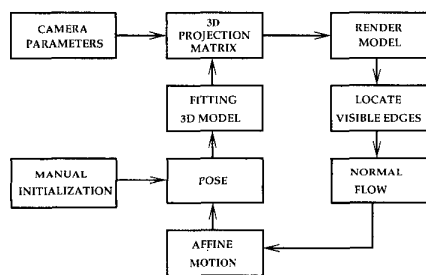
Figure 2: The tracking system.
